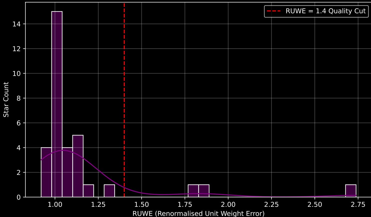
GALAH DR4 Field [-7] RUWE Distribution (n= 33)
