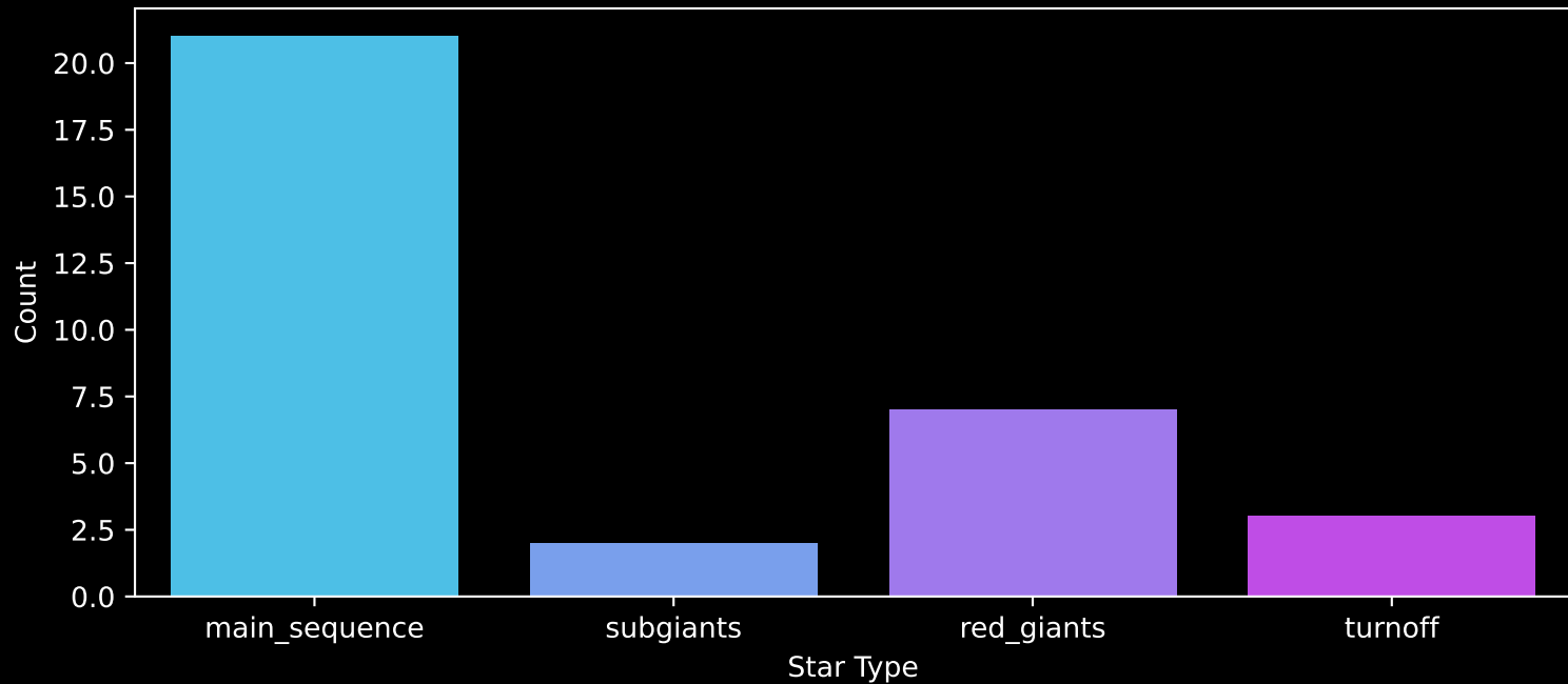
GALAH DR4 Field: [-7] Count plot of Star Type
