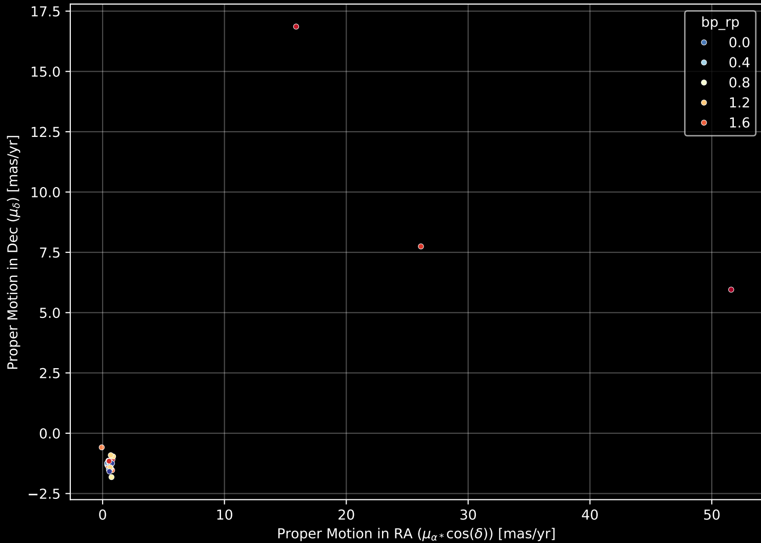
GALAH DR4 Field: [-7] Proper Motion Diagram (n= 33)
